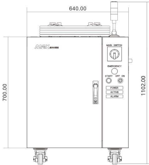
Laser Three Views. (Unit: mm)
